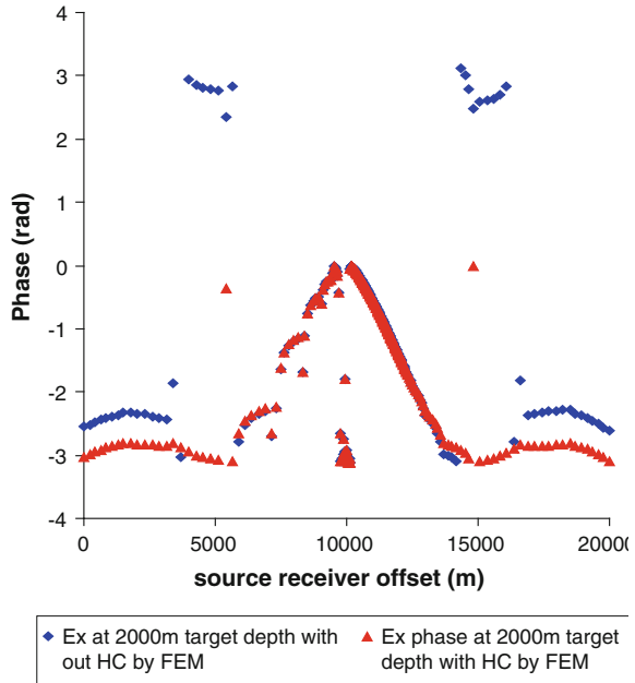
Fig. 20 PVO with and without HC at 2000 m target depth using FEM
