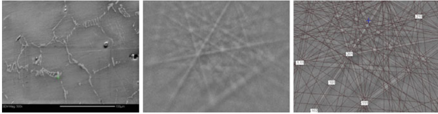
Fig. 5 Experimental EBSD pattern obtained from the lamellar phase indexed as Al_4Sr (tetragonal crystal structure), Mean angle of deviation (MAD) = 0.59^\circ , orientation = (151.4, 93.8, 11.5^\circ ), spec. plane (-5-10)
