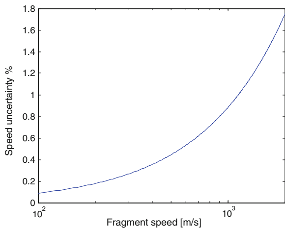
Fig. 6 Speed timing uncertainty dependent on actual speed
