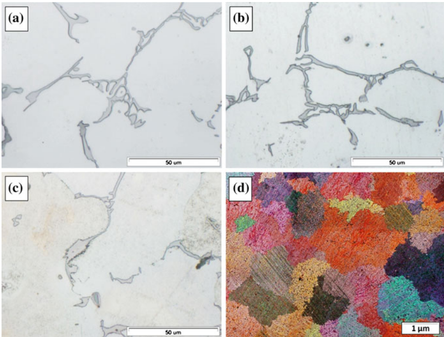
Fig. 6 Examples of revealed microstructures after etching with different reagents: 25 ml H_2O , 75 ml ethylene glycol, 1 ml HNO_3 in bright field, low quality for detection of phases (a); 5–20 ml acetic acid, 80–95 ml H_2O in bright field, good quality for detection phases (b); 4.2 g picric acid, 10 ml acetic acid, 10 ml H_2O , 70 ml ethanol in bright field, very low quality for detection of phases (c); 4.2 g picric acid, 10 ml acetic acid, 10 ml H_2O , 70 ml ethanol in polarized field with quarter-wave plate, good quality for detection of grain boundaries (d)
