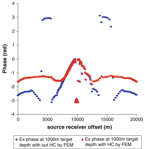
Fig. 18 PVO with and without HC at 1000 m target depth using FEM
